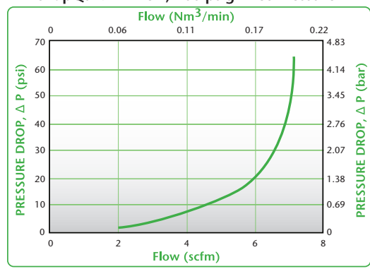
SnapQuik Air Flow, 100 psig Inlet Pressure
