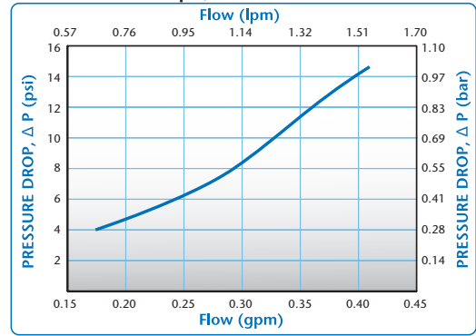
SnapQuik Water Flow
